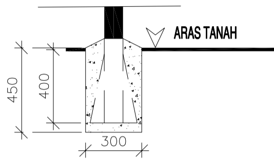
BUTIRAN A NOT TO SCALE
