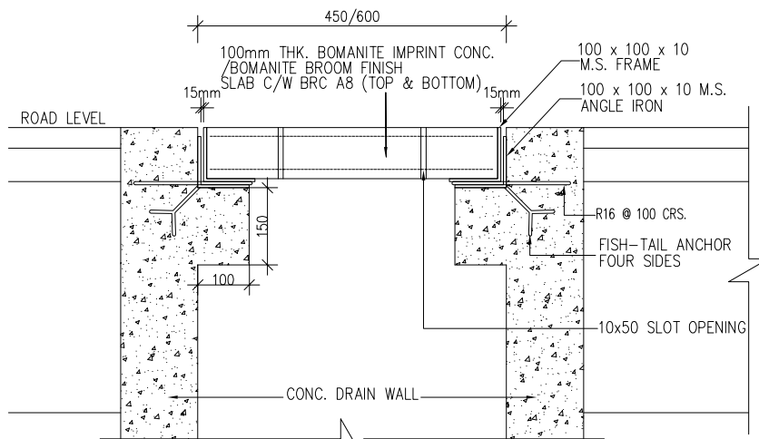
SECTION VIEW OF PROPOSED CONC. SLAB COVER (WITHOUT TRAFFIC LOADING)
