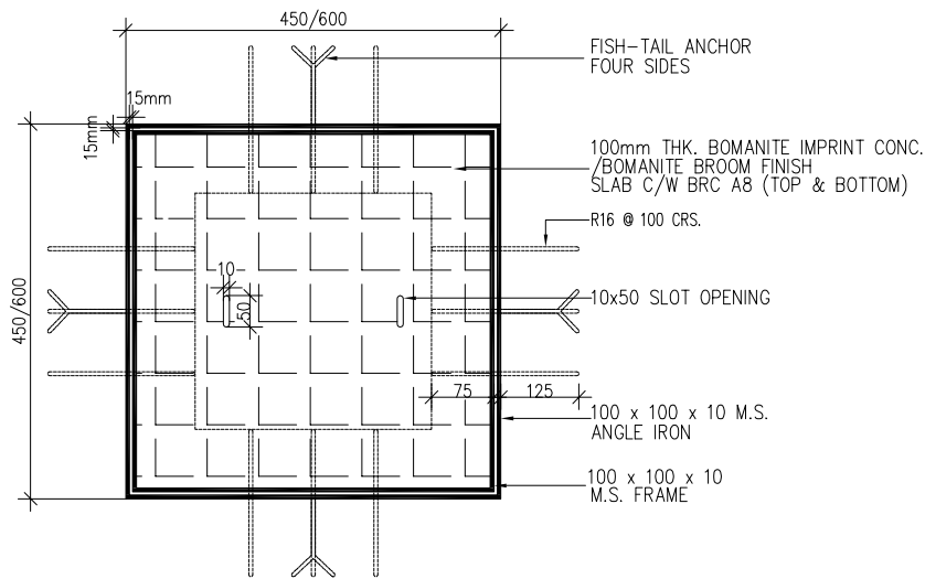
PLAN VIEW OF PROPOSED BOMANITE BROOM FINISH CONC. SLAB COVER FOR DRAIN/SUMP AT 6m C.C (WITHOUT TRAFFIC LOADING)
