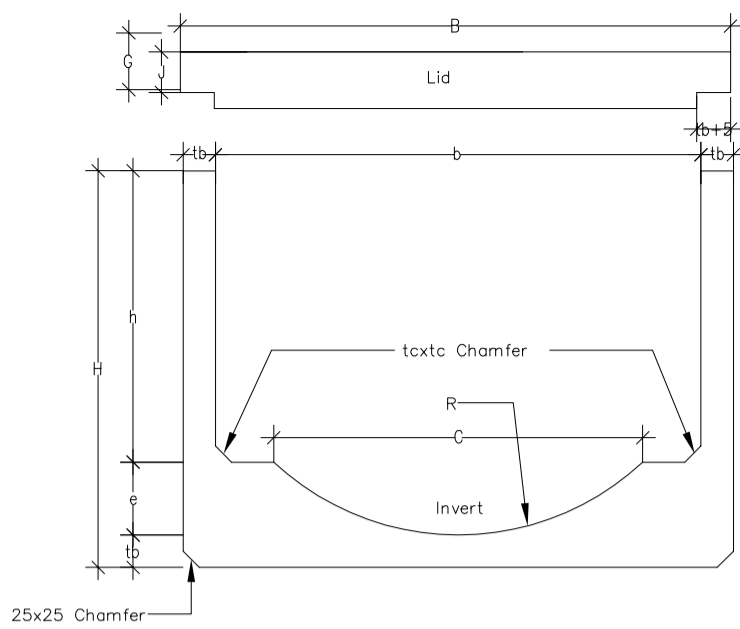
BUTIRAN KERATAN RENTAS 'PRECAST BOX CULVERT WITH DRY WEATHER FLOW'
