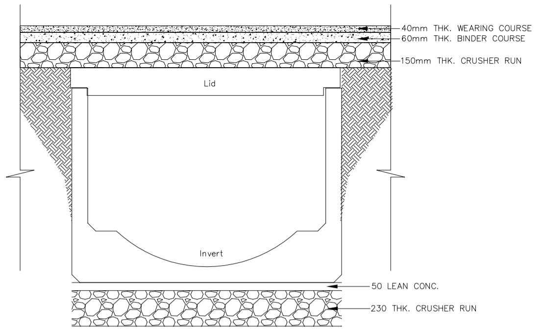
BUTIRAN PEMASANGAN 'PRECAST BOX CULVERT WITH DRY WEATHER FLOW'
