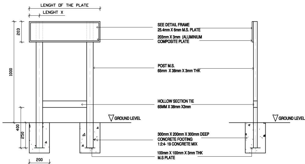
FRONT ELEVATION
