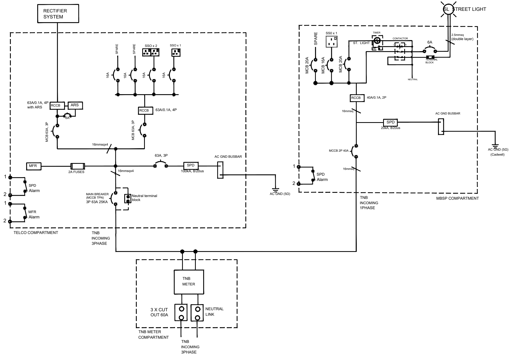
ELECTRICAL SCHEMATIC DIAGRAM
